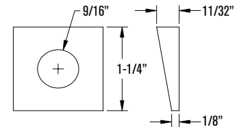
HARDWARE SHIM
