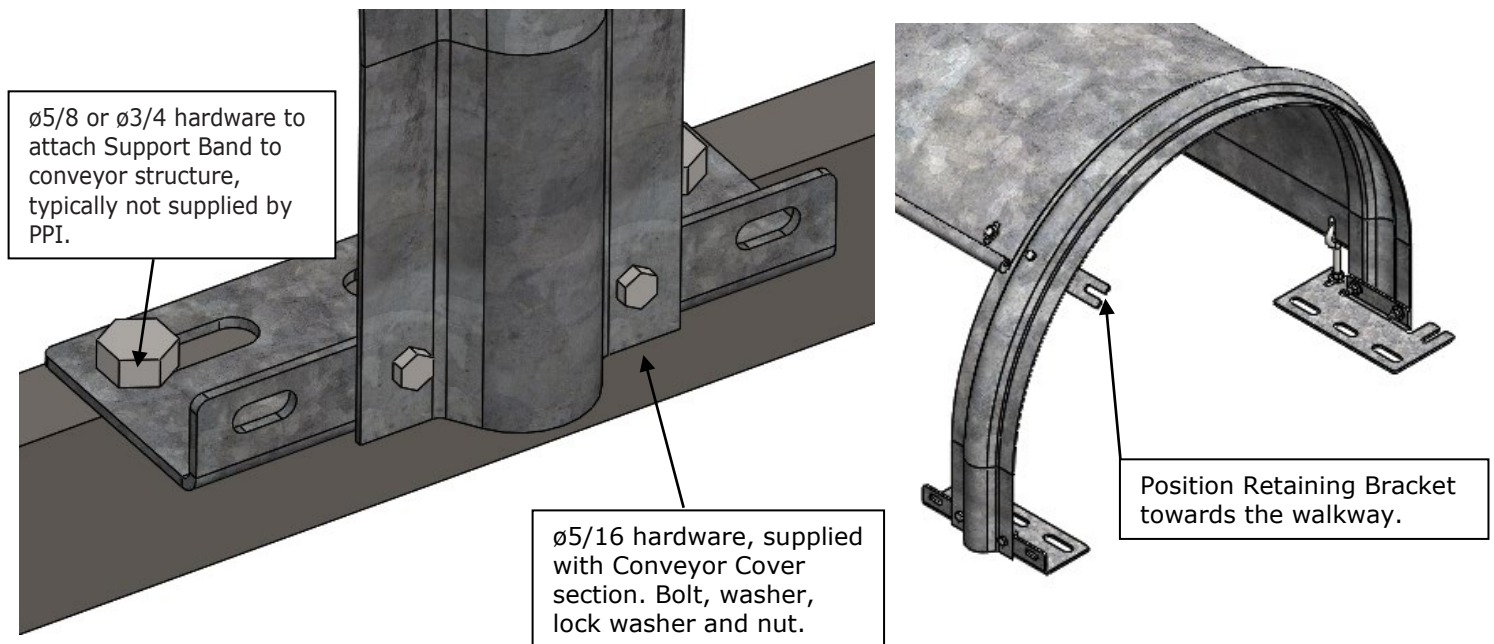
Figure 10: ATTACHING FOOT SUPPORT BRACKET 3/4 TO CONVEYOR STRUCTURE
