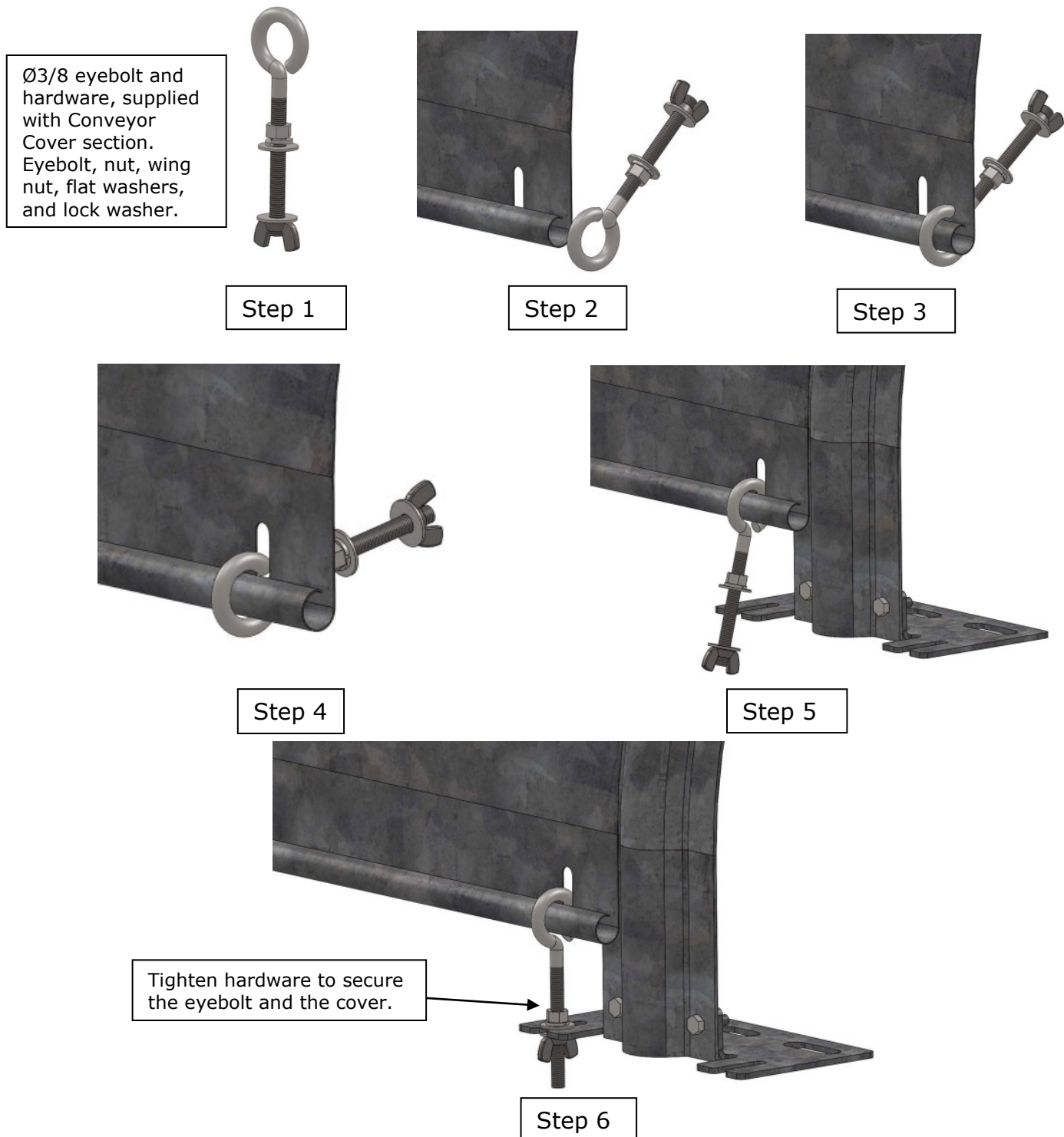
Figure 11: FULL COVER SECTION ASSEMBLY
