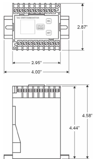
FIGURE A5 .5: 47268 Smart Monitor dimensions.
