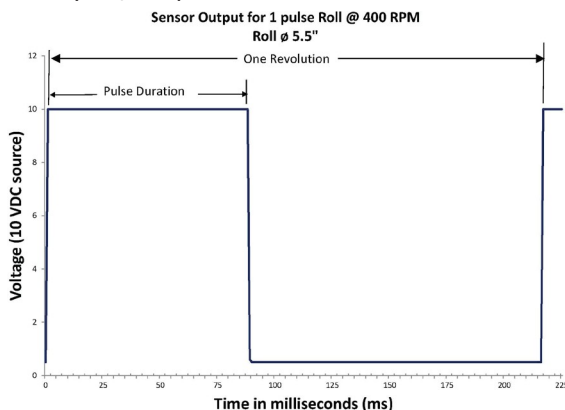
Figure 6.1: Example sensor output for a 1 pulse roll, P/N SAD5CSRSB-1PL4
