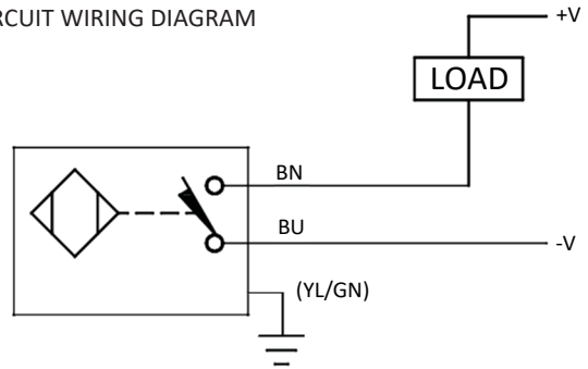
FIGURE A4.2: 2 WIRE DC SINKING (NPN) CIRCUIT WIRING DIAGRAM
