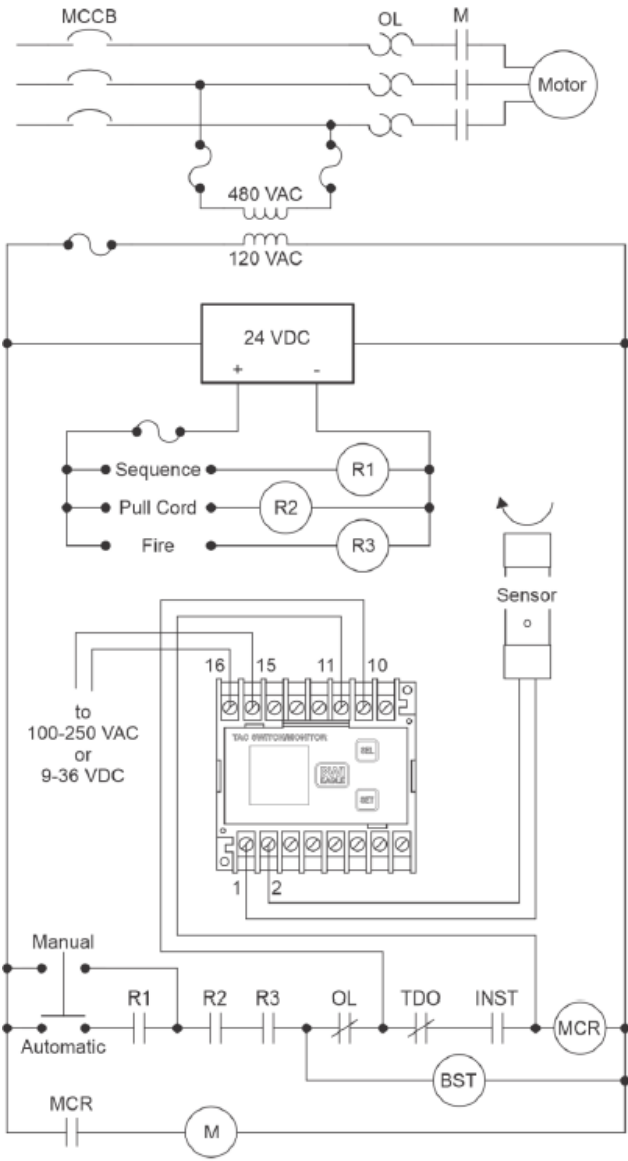
Figure 4.3 Sample Wiring Diagram
