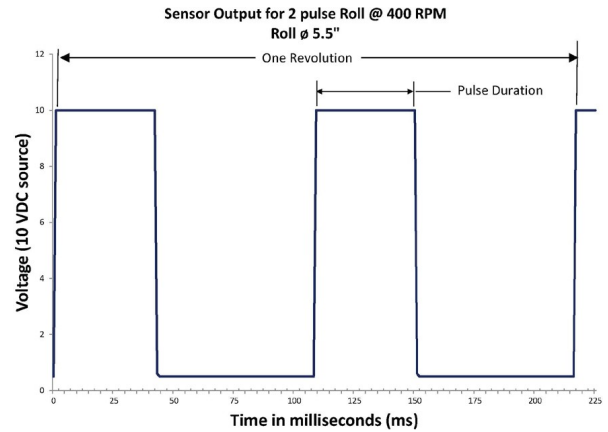
Figure 6.2: Example sensor output for a 2 pulse roll, P/N SAD5CSRSB-2PL4
