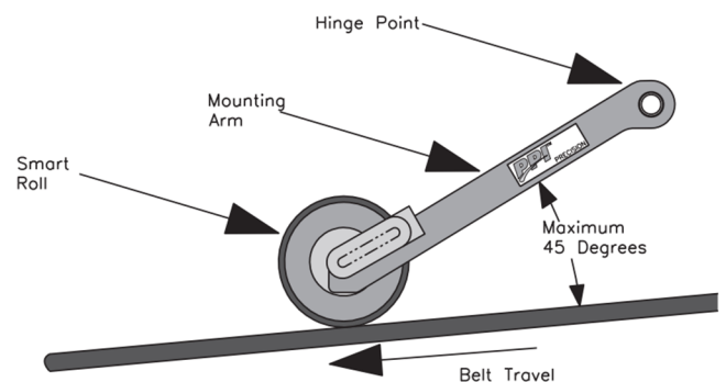
FIGURE 2.2: CSR Mounting
