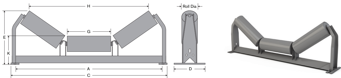
CEMA D EQUAL TROUGHERS
