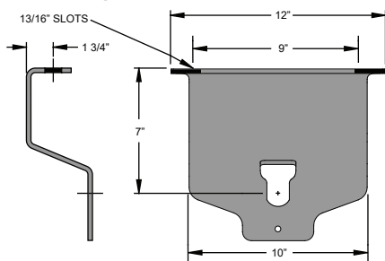
7" E - Drop Bracket (standard) - #41210
