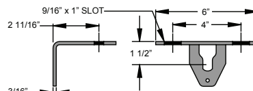
B,C - 1½" Drop Bracket (optional) - #02200
