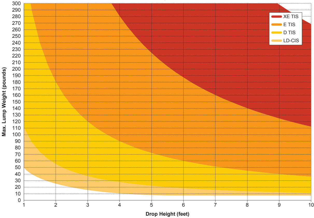
Impact Loading Selection Chart
