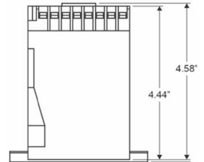
FIGURE A5 .5: 47268 Smart Monitor dimensions.
