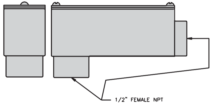
FIGURE 3.1: 90° Elbow Conduit Access Port
