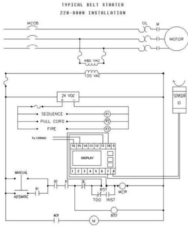
Figure 4.3 Sample Wiring Diagram
