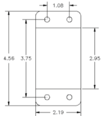
FIGURE A5.8: 47269 Smart Monitor dimensions.
