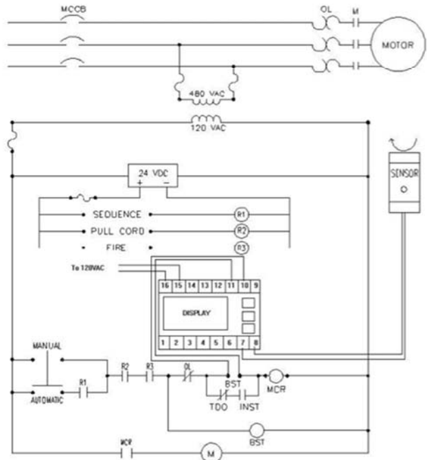
TYPICAL BELT STARTER 220-8000 INSTALLATION
