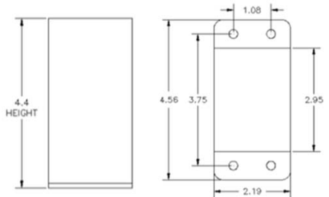
FIGURE 4.1: 37543 Smart Monitor dimensions.
