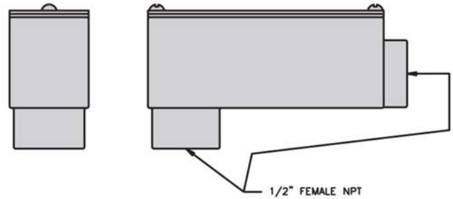
FIGURE 3.1 90° Elbow Conduit Access Port.
