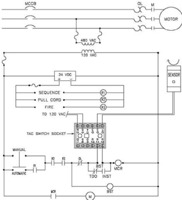
TYPICAL BELT STARTER 22-8000 INSTALLATION
